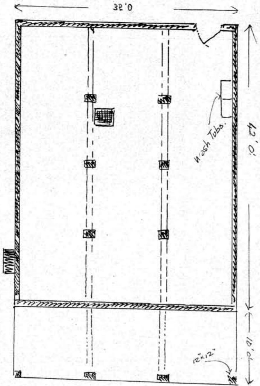
Foundation Plan.
