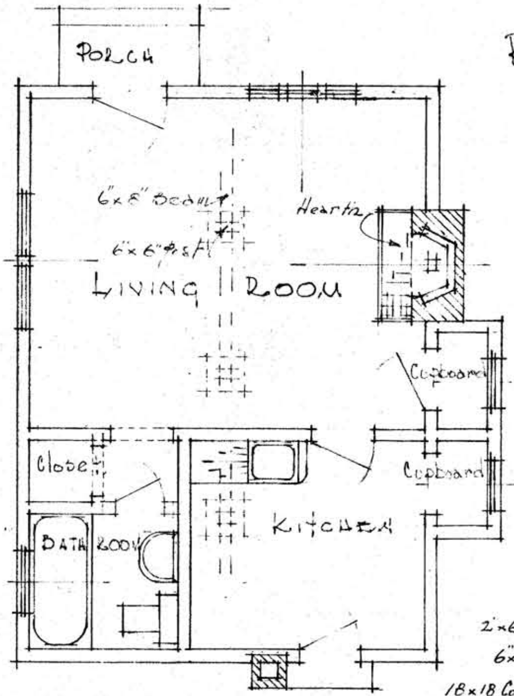
FLOOR PLAN
