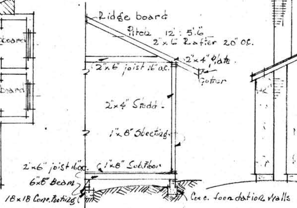
SECTION
