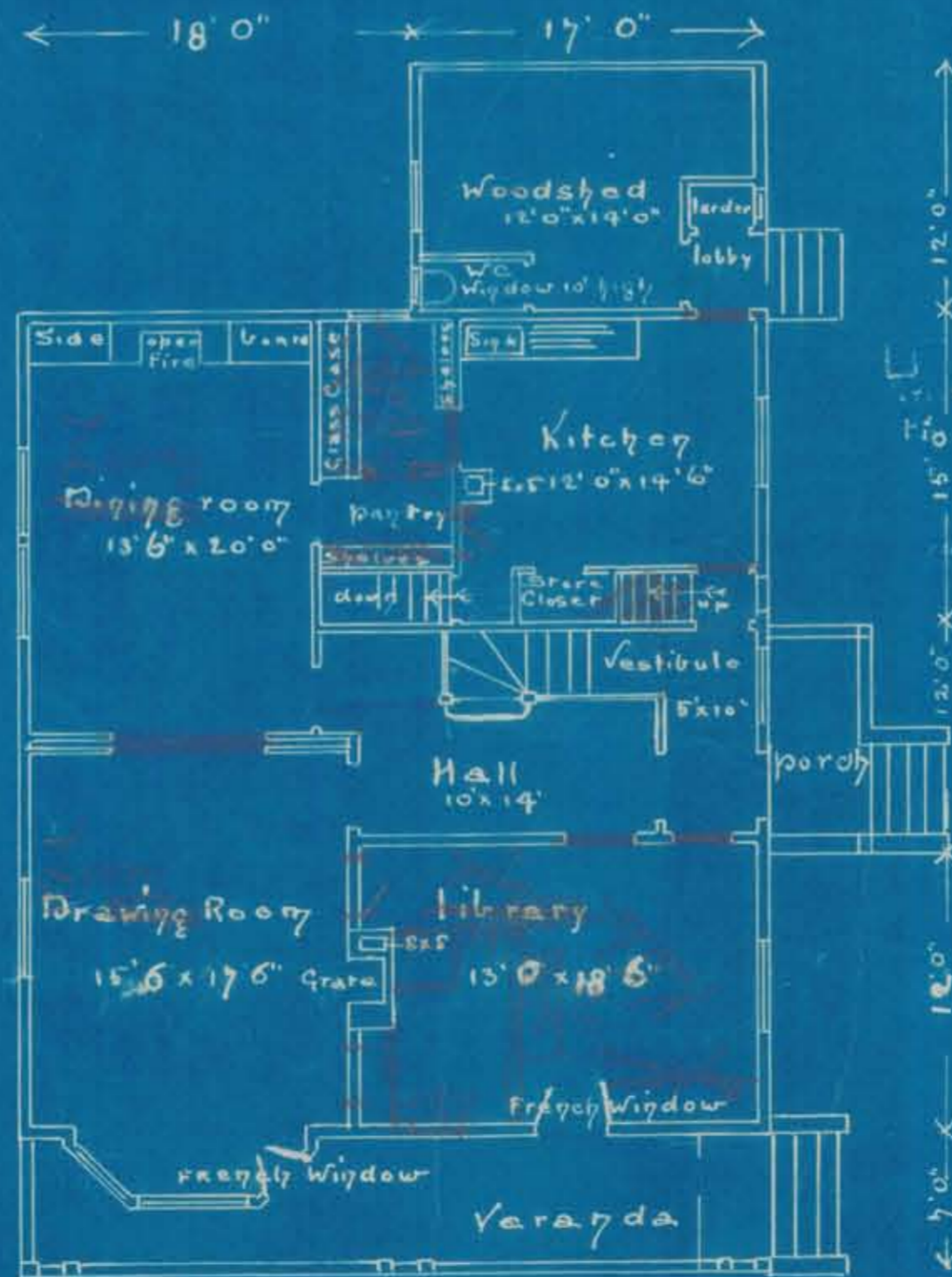
First Floor plan Scale 1/8" = 1 foot
