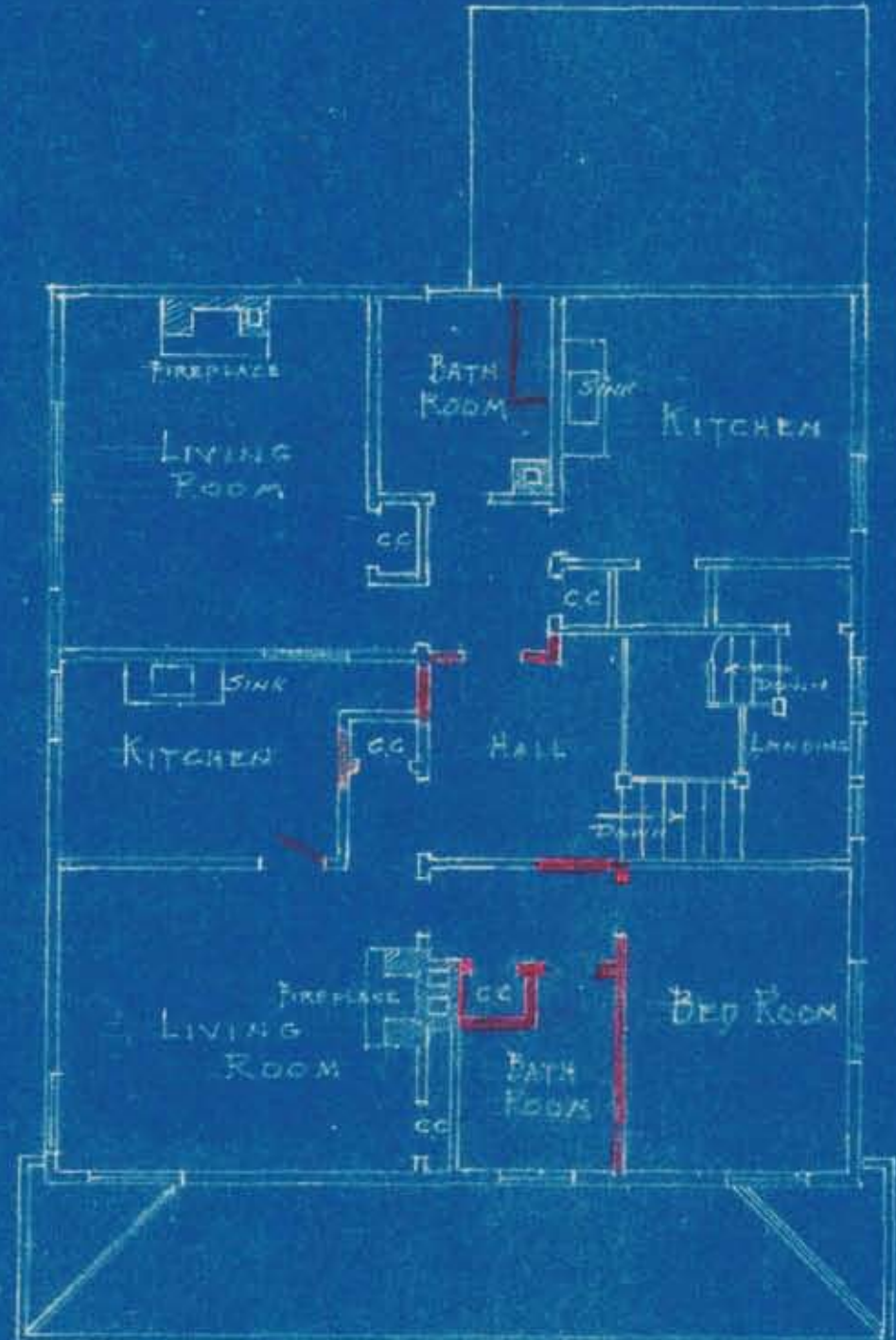
SECTION FIRST FLOOR PLAN
