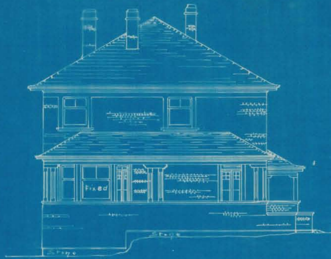
South Elevation
