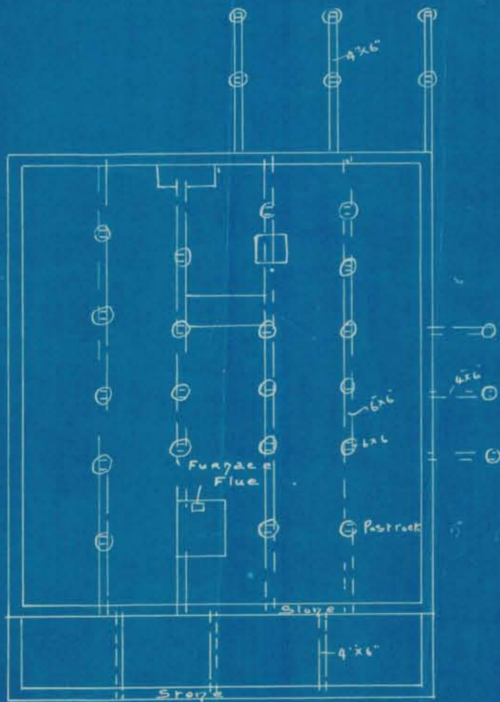
Foundation plan
