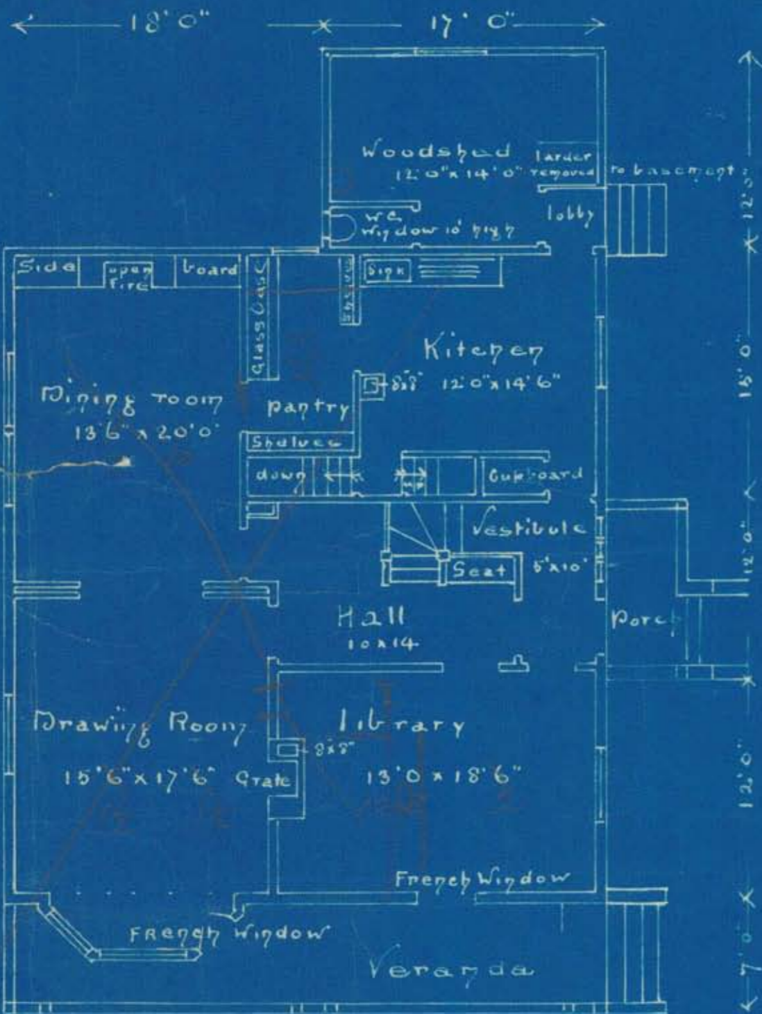
First Floor plan Scale + one foot
