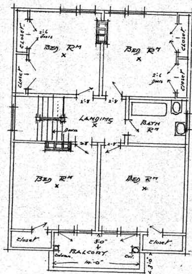
BED ROOM PLAN.
