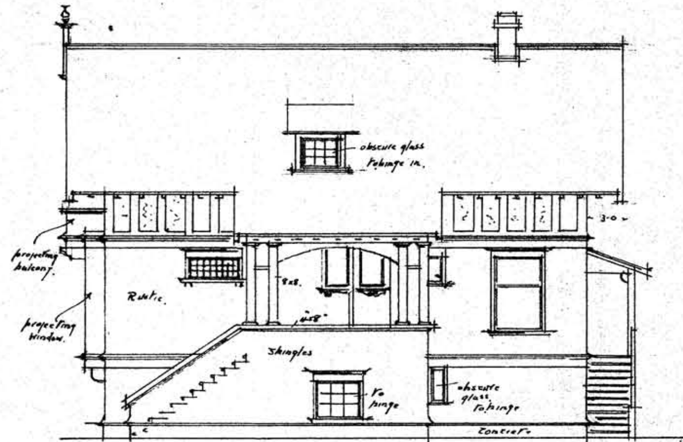
SIDE ELEVATION.
