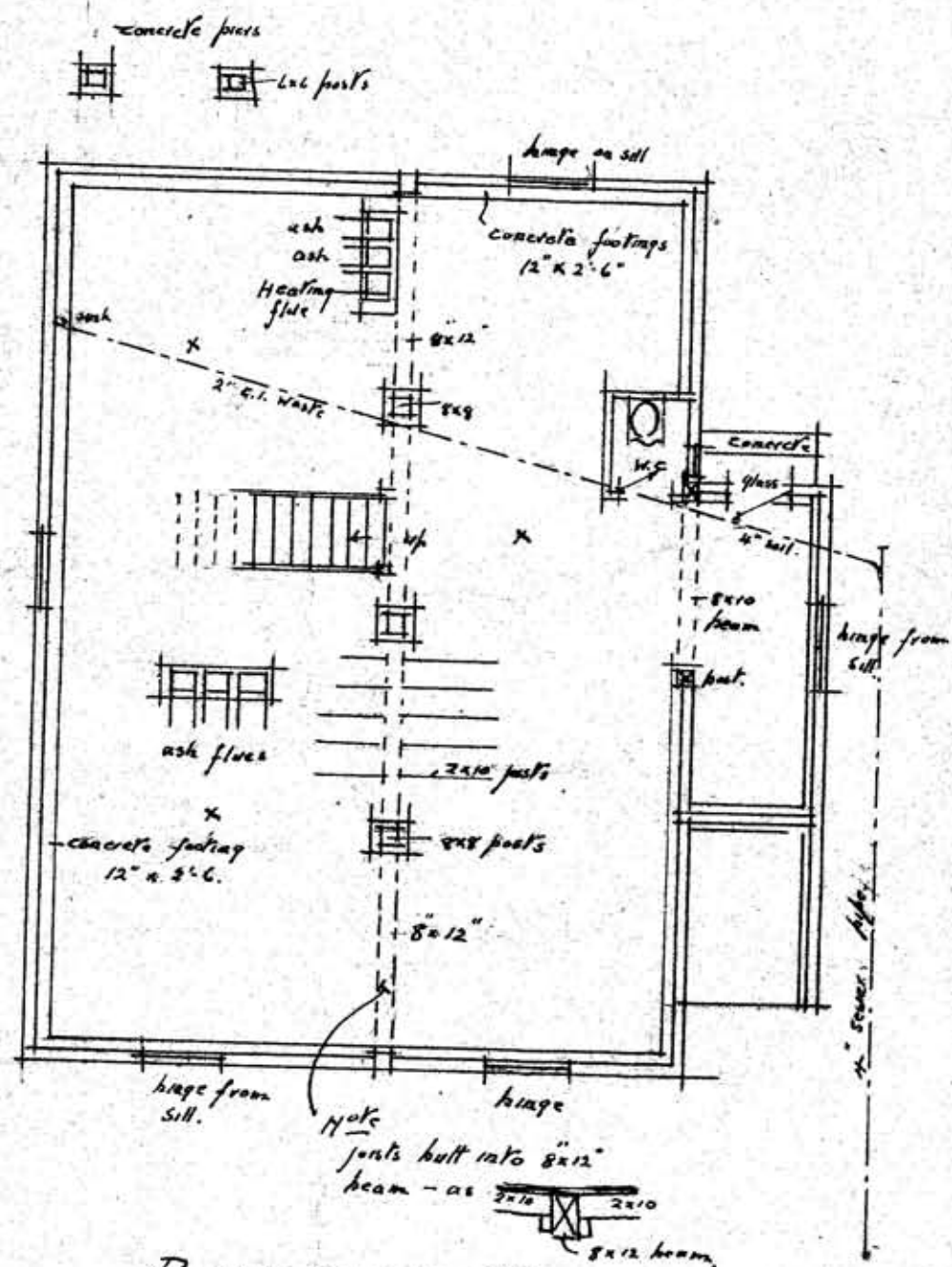
BASEMENT PLAN.
